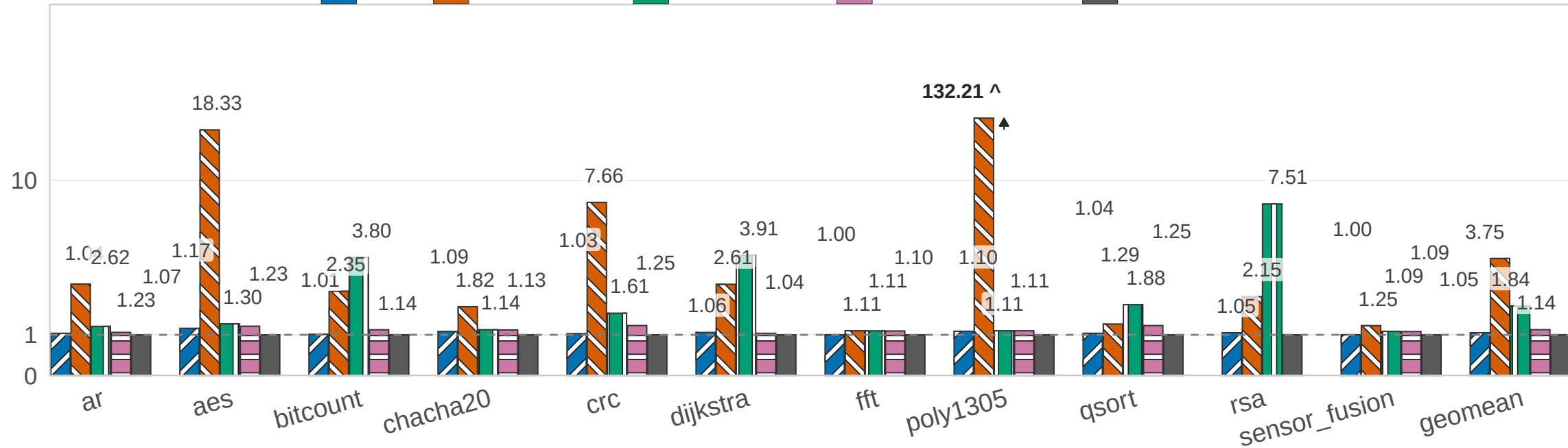
Relative Execution Time
