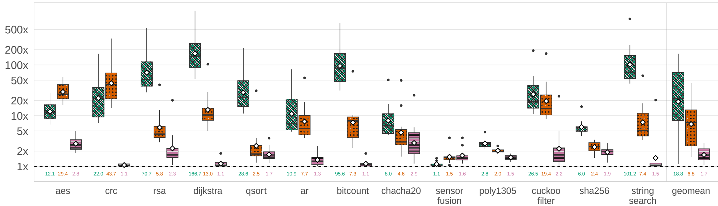
Relative Execution Time (to BAO)
