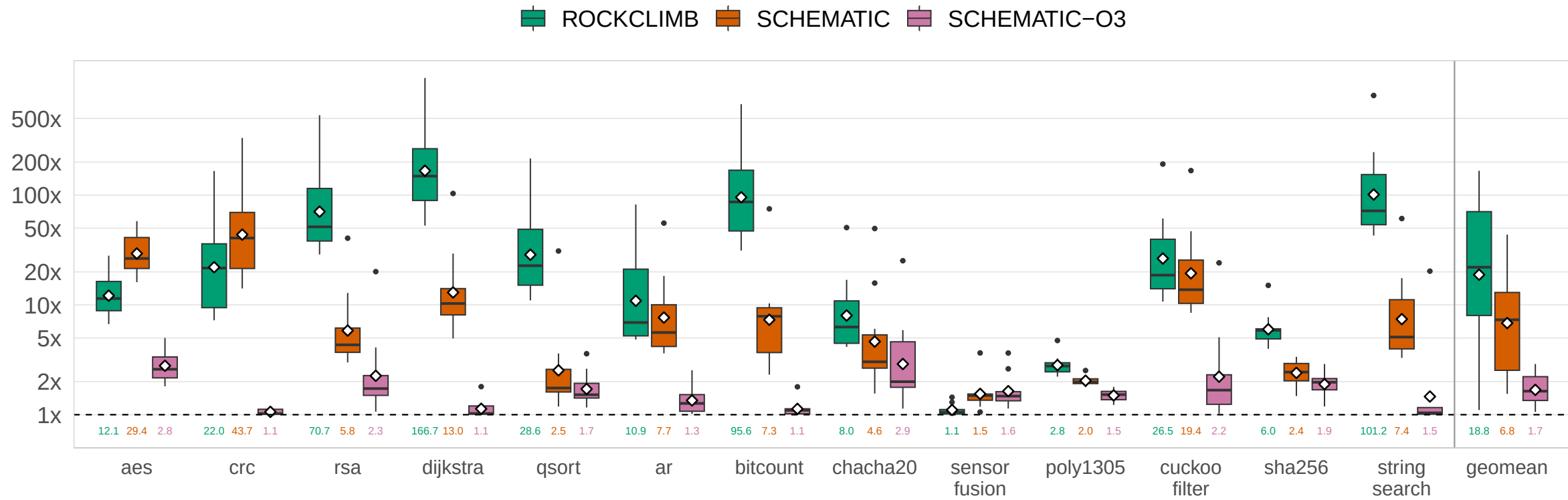
Execution time normalized to BAO
