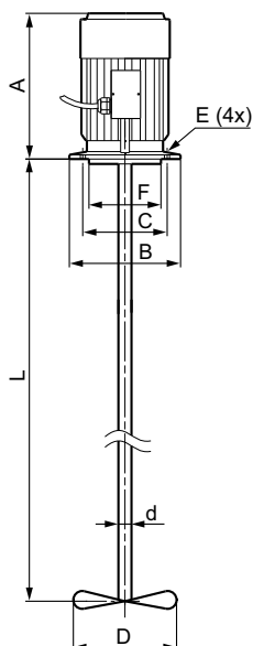
Fig. 2 Stainless steel version* with propeller as mixer
