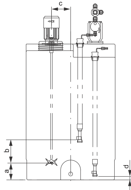
Fig. 4 Installation sketch
