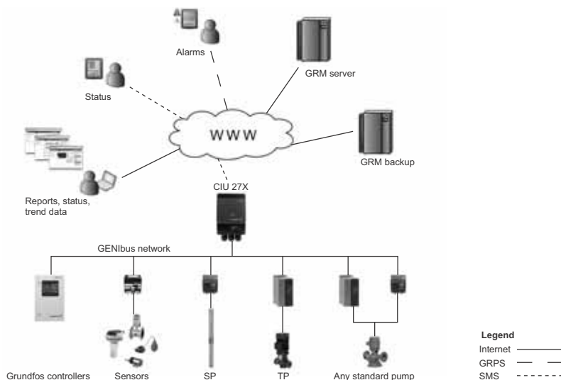
Fig. 1 Grundfos Remote Management
