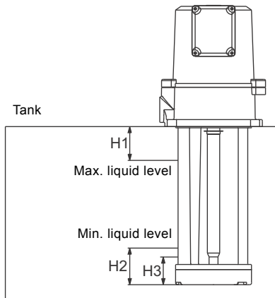
Fig. 5 MTA with top suction
