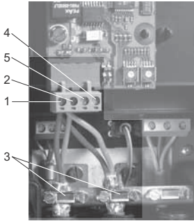
Fig. 2 Connecting the Profibus
