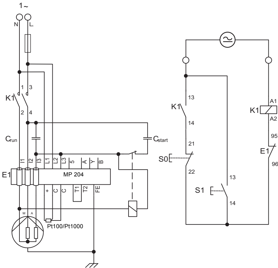
Fig. 4 Single-phase connection
