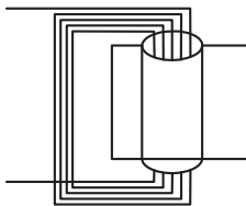
Fig. 3 Five windings per phase through MP 204
