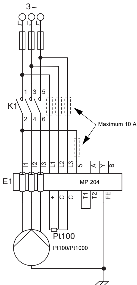
Fig. 1 Three-phase connection
