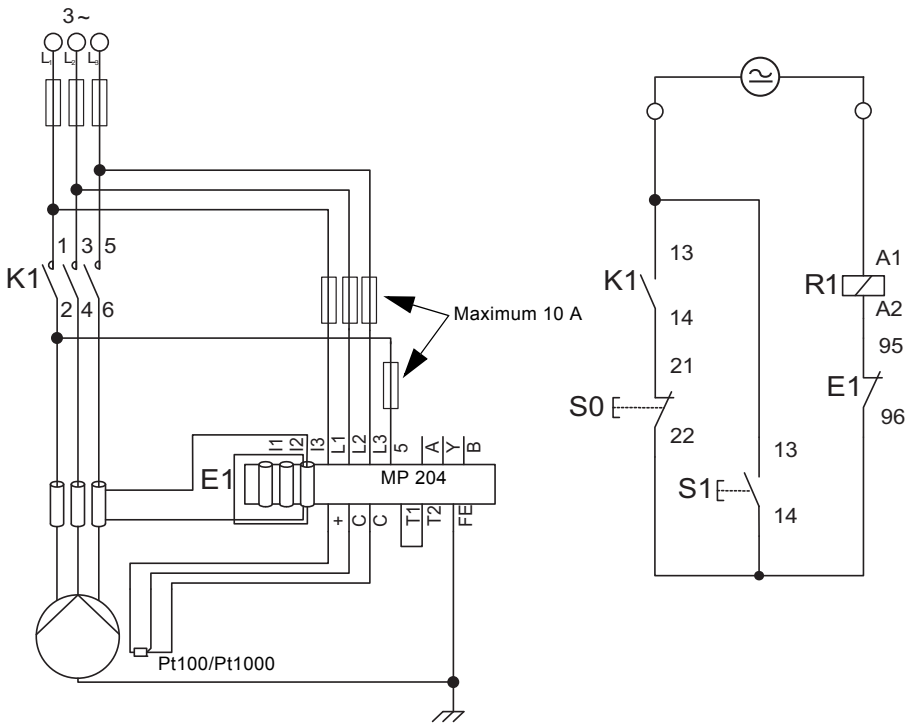
Fig. 2 Three-phase connection with current transformers
