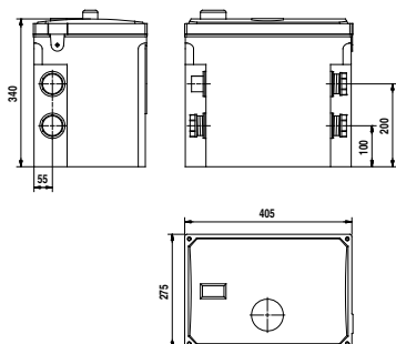
Fig. 2 Dimensional sketches
