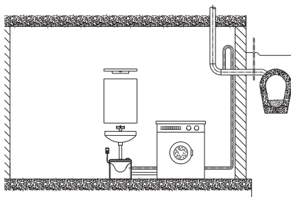
Fig. 3 Installation example
