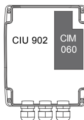
Fig. 2 Position of the CIM 060 in a CIU 902
