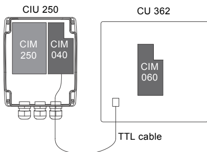
Fig. 5 CIM 060 in a CU 362 connected to a GSM network
