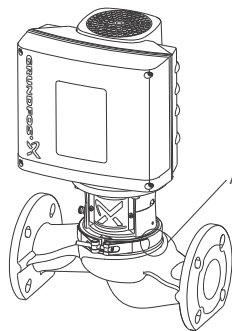
Fig. 3 Clamp (A)
