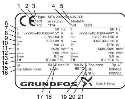
Fig. 1 Example of nameplate
