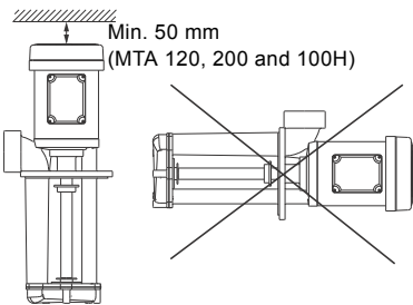
Fig. 2 Mounting position
