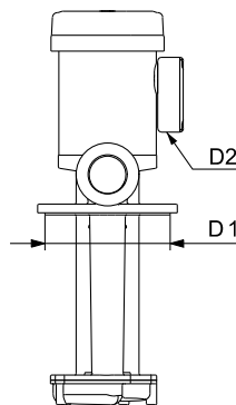
Fig. 4 Tank hole and cable entry
