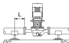
Fig. 6 Pump suspended directly in the pipes
