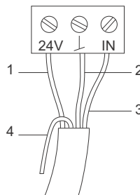
Fig. 2 Wiring diagram for temperature measurement
