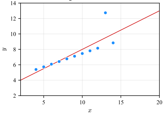
III: a tight line and one outlier
