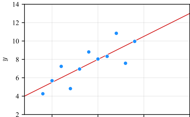
I: a linear relation with scatter
