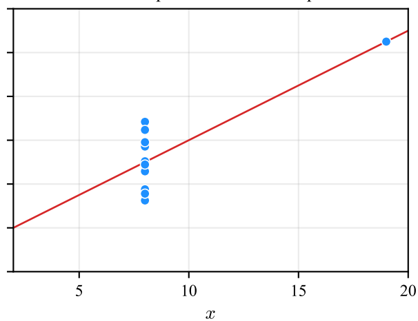
IV: one point decides the slope
