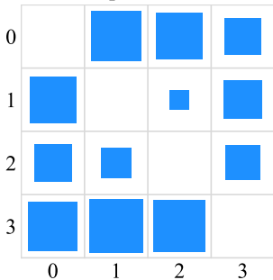
(a) Hinton square area
