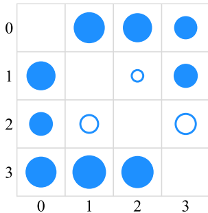
(b) bubble grid circle area
