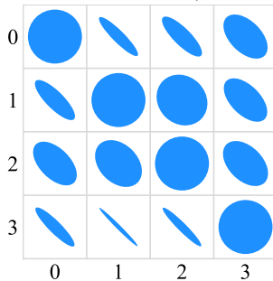
(c) corrplot ellipse eccentricity
