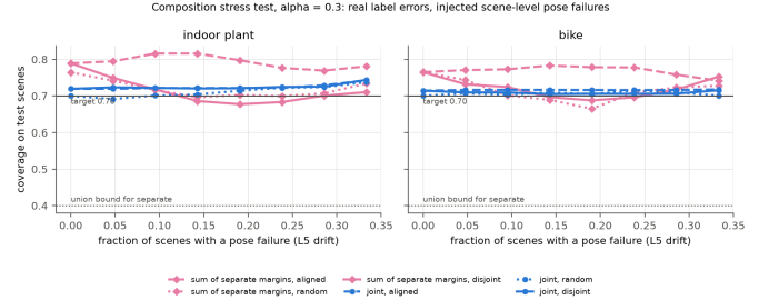
Fig. 2. Coverage of the sum of separate margins and of the joint margin vs. the fraction of scenes with a localization failure placed where labels are worst (dashed), best (solid) or at random (dotted); 1 - \alpha = 0.7 .
