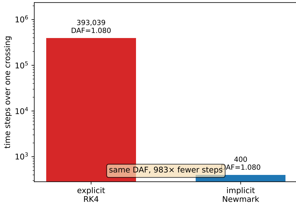
(b) cost on the damped 40 m bridge
