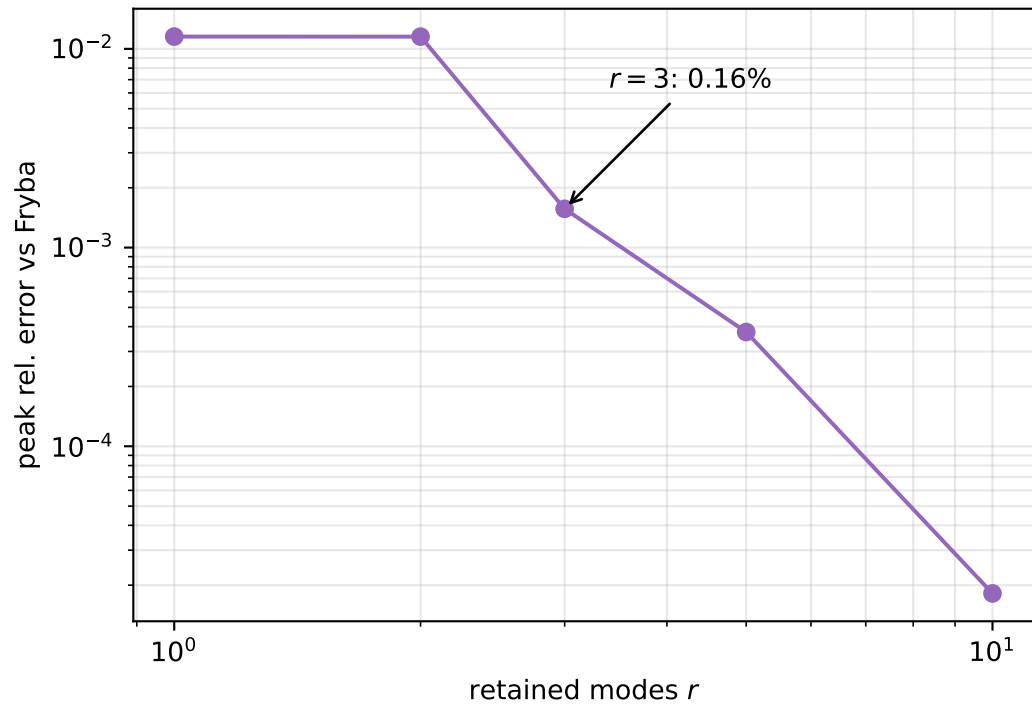
(a) modal truncation convergence (20 m)
