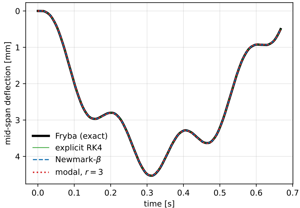
(a) 20 m beam: all methods vs Fryba
