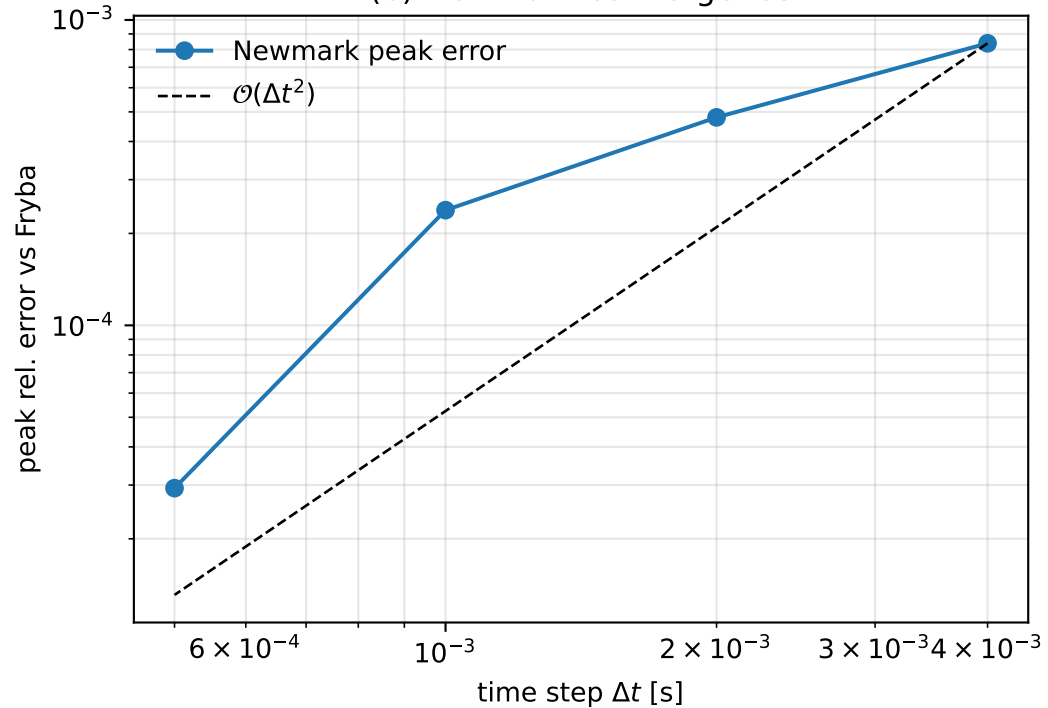
(b) Newmark convergence
