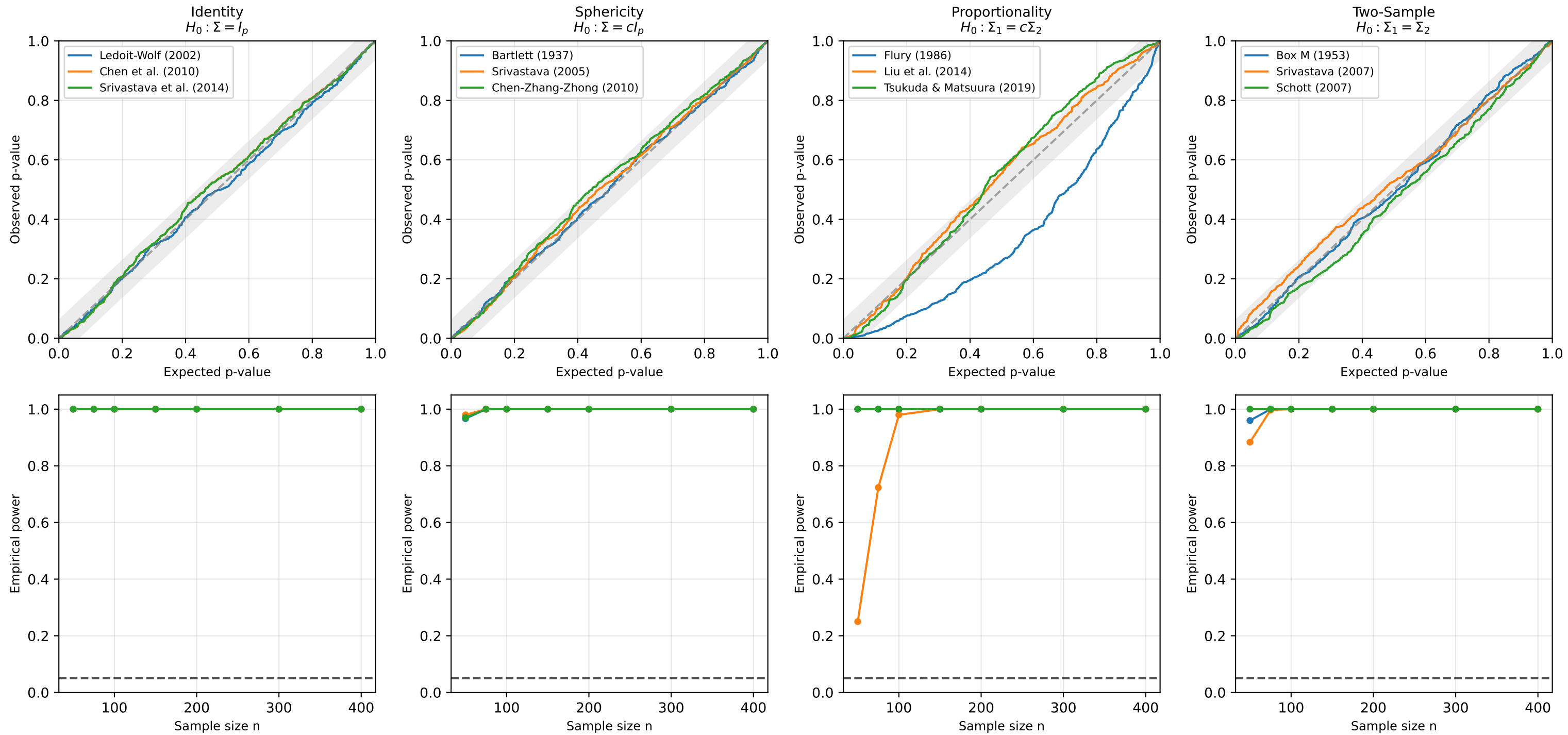
Null Calibration (top) and Power (bottom) for Four Covariance Test Classes
