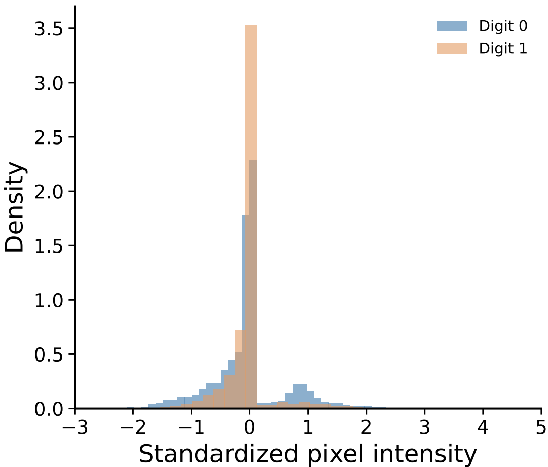
MNIST input distributions
