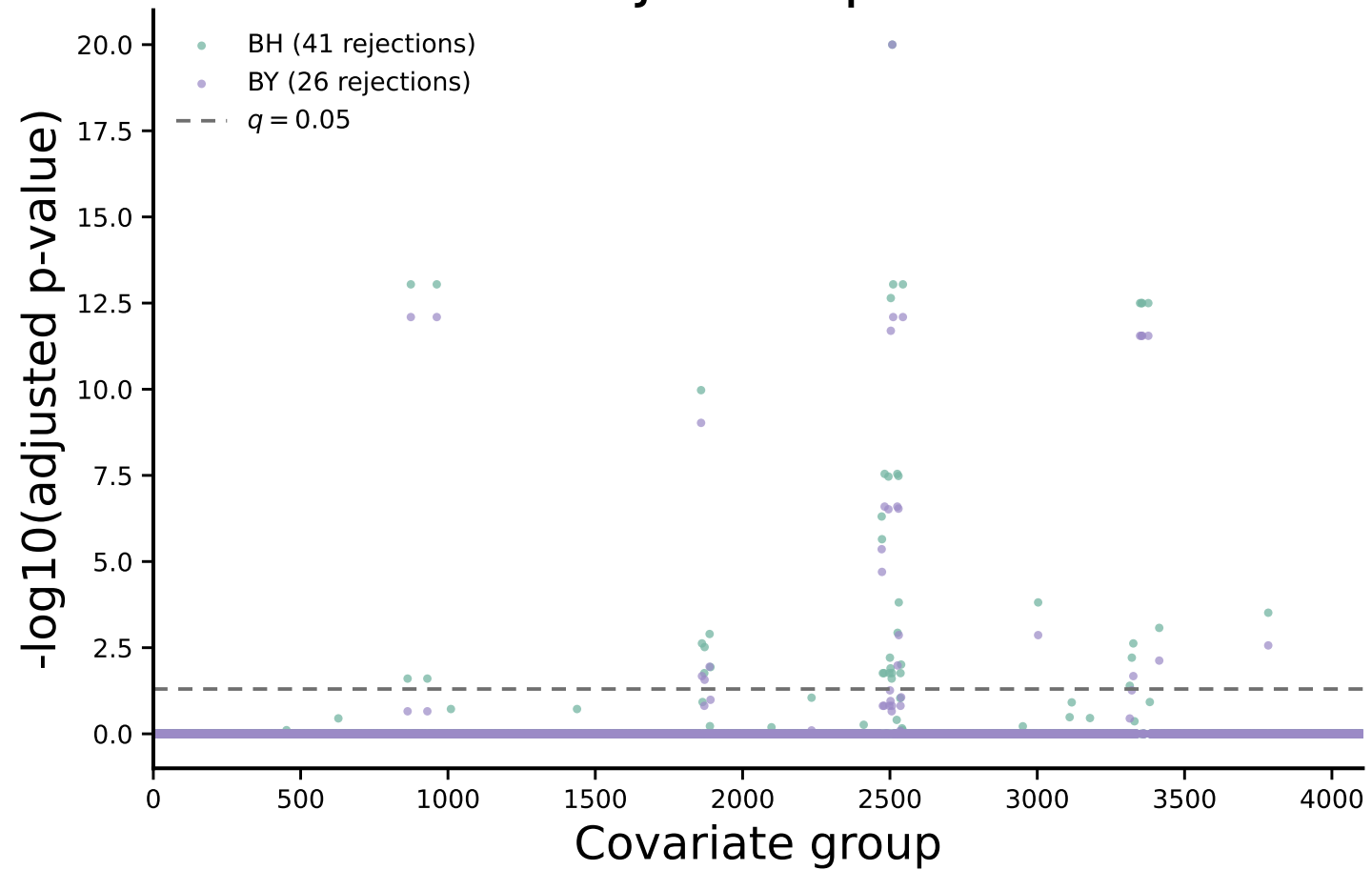
FDR-adjusted p-values
