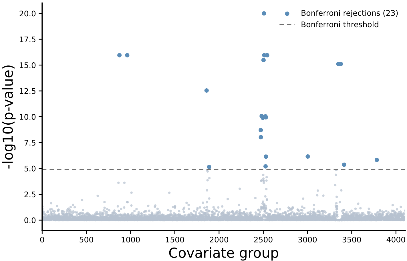
Block-level p-values
