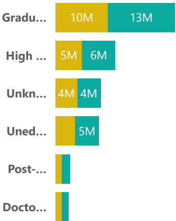
Revenue by education lvl
