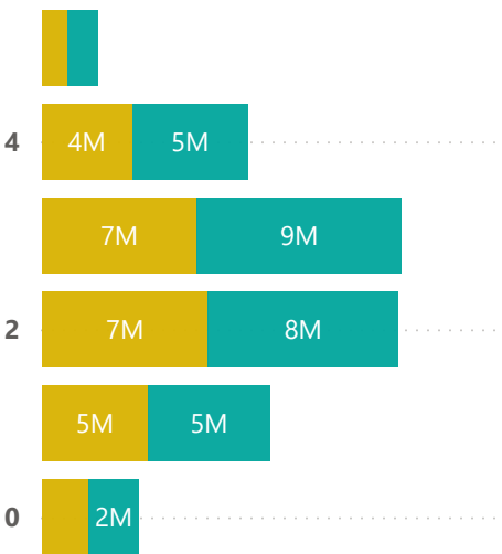
Revenue by Dependent cnt
