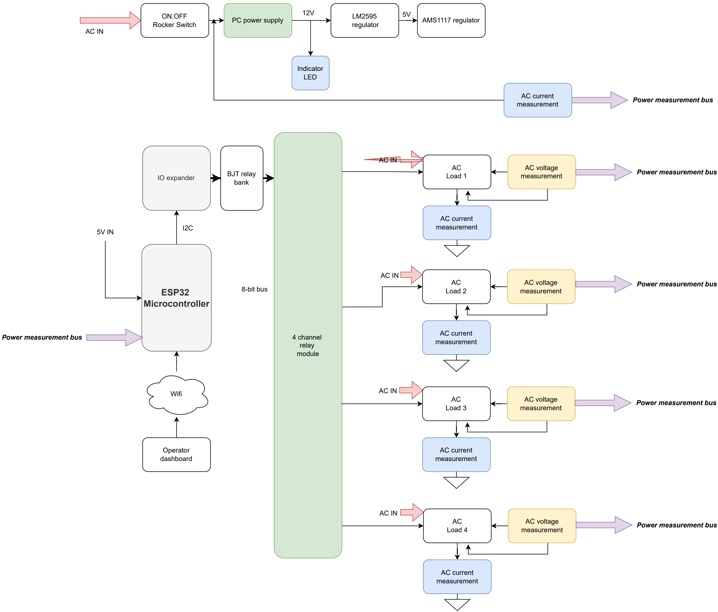
Load Management System Block Diagram
