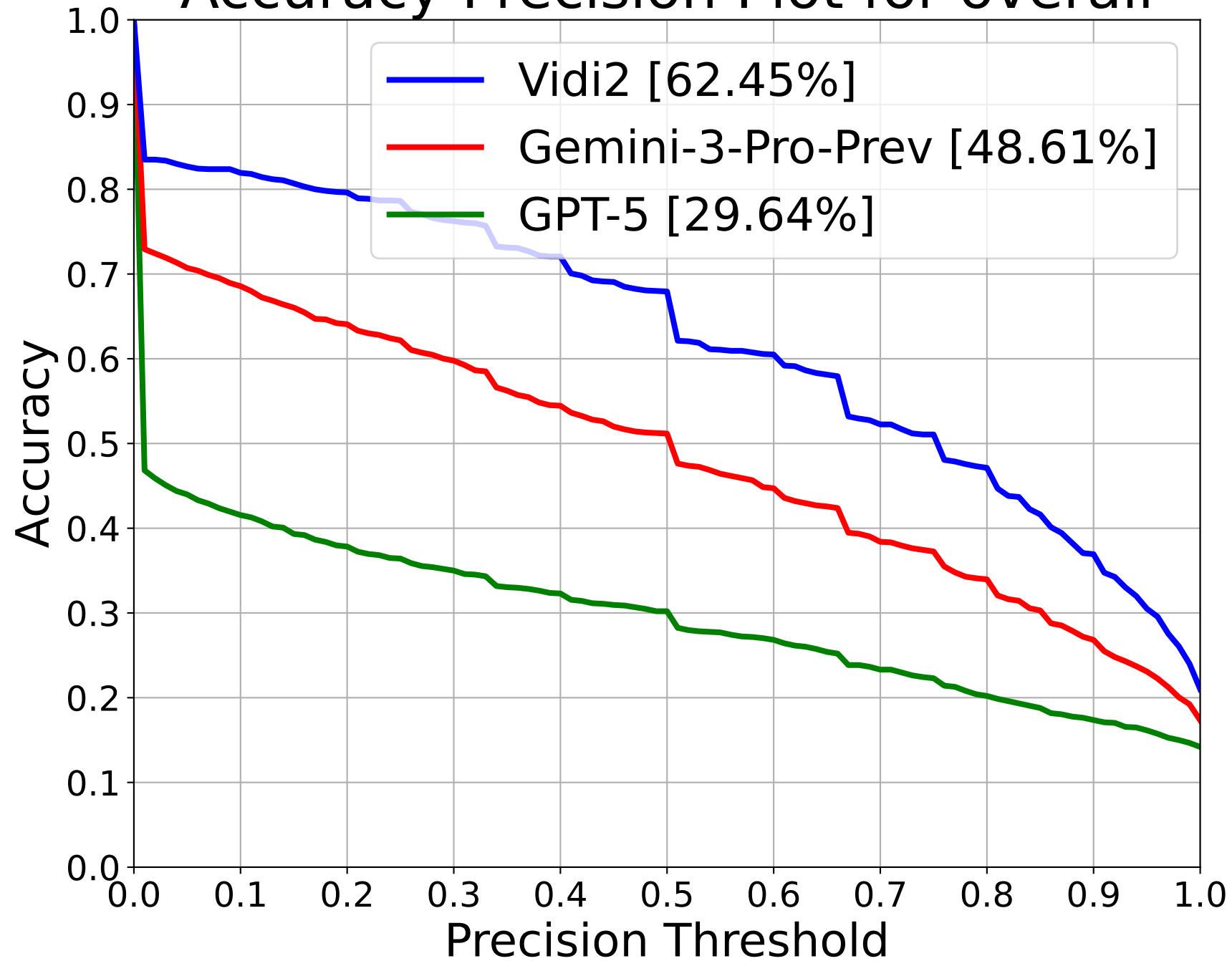
Accuracy-Precision Plot for overall
