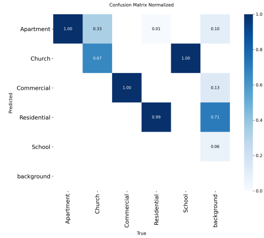
(b) Normalized confusion matrix
