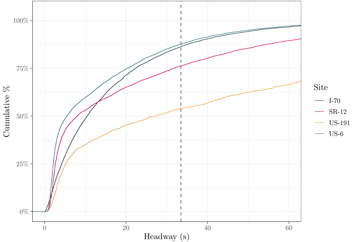
Figure 7: Cumulative distribution of headways at each site, with critical headway marked as a vertical line.
