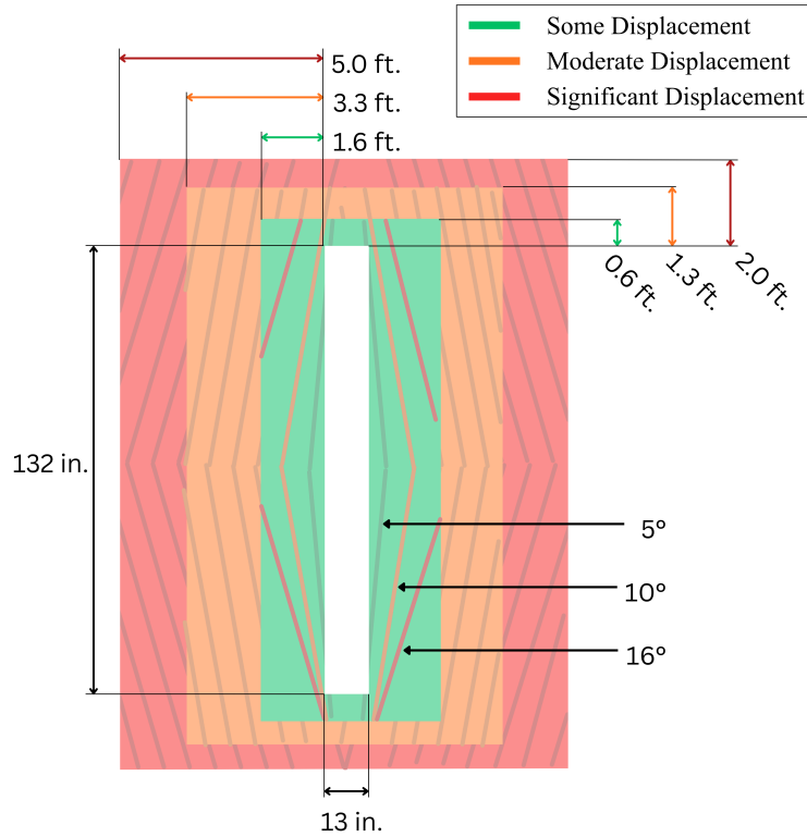
Figure 3: TPRS displacement overlay.
