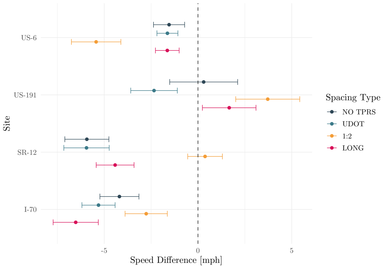
Figure 5: Change in 85th percentile speed between radar speed units with 95 percent confidence interval on difference in speeds.
