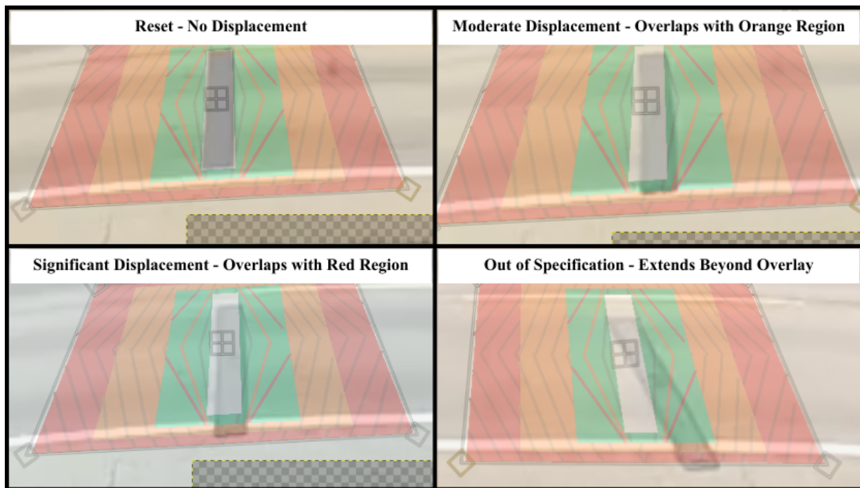
Figure 4: TPRS displacement examples.
