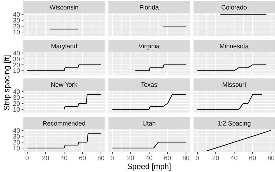
Figure 1: Various specifications for TPRS spacing.
