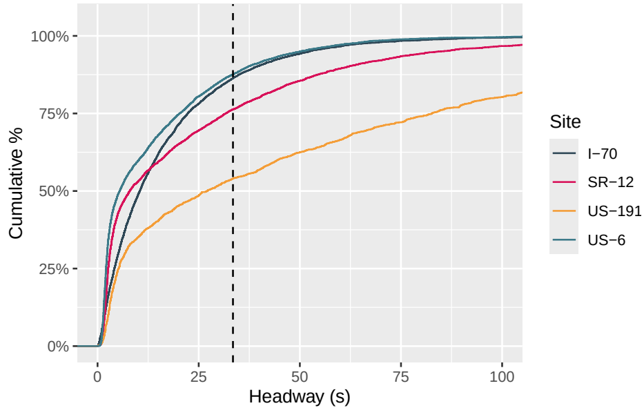
Figure 9: CDF of headways for each site.
