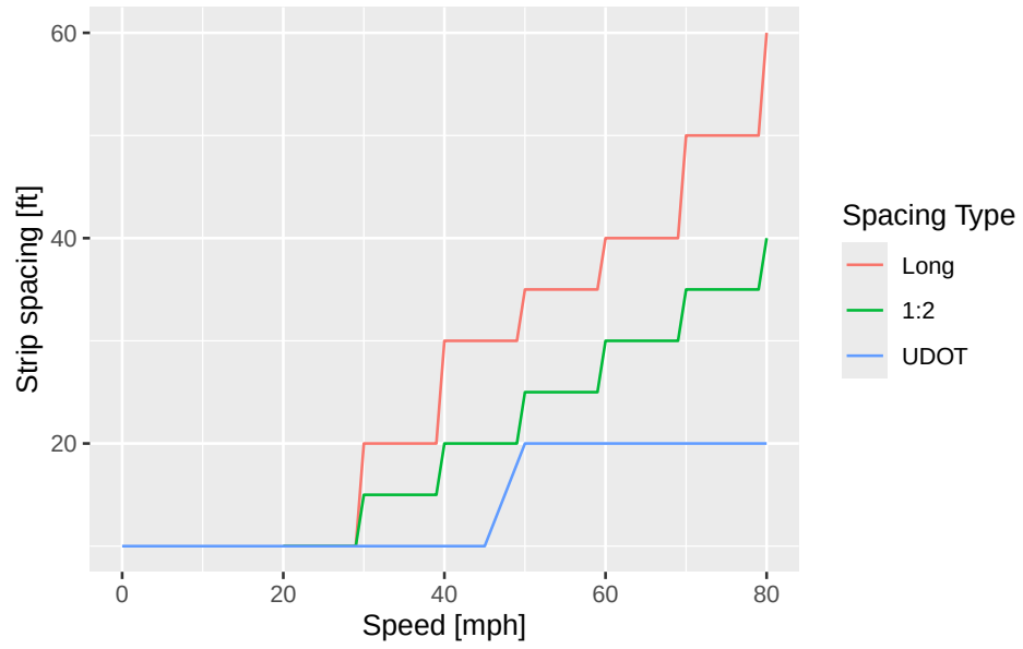
Figure 4: Spacing specifications used in testing.
