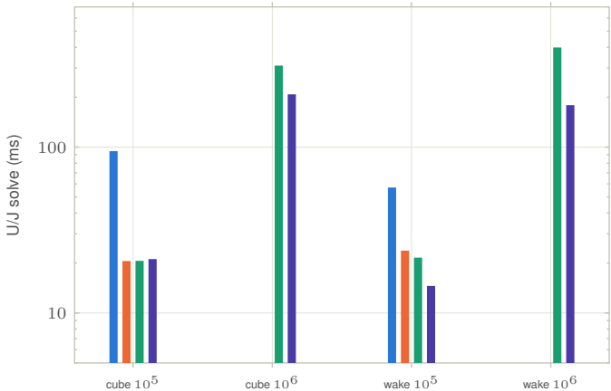
(b) Float64
