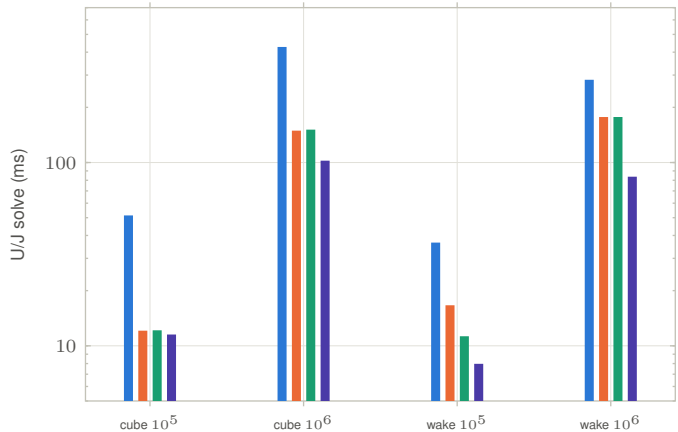
(a) Float32
