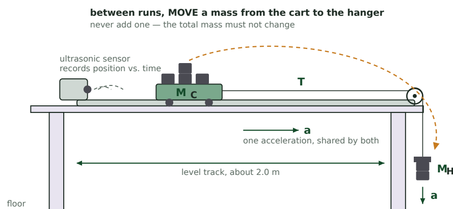
Figure A. The half Atwood machine. One light string runs from the cart over the pulley at the table edge and carries a single tension T throughout. The cart and everything on it, plus the hanger and everything on it, form one system of total mass M_T moving with one acceleration a — which is why the same letter labels the arrow on the track and the arrow below the hanger. The orange path is the procedure that makes the experiment work: mass is moved from cart to hanger between runs, so the driving force F_{g,H} = M_H g rises while M_T stays exactly the same.
