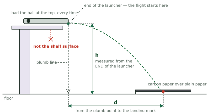
Figure A. Where the two measurements are taken. h runs from the end of the launcher to the floor — not from the shelf surface, which sits lower and will bias every prediction you make. d runs from the point directly below the launcher end, found with a plumb line, to the landing mark. Your own report needs a photo of your apparatus and a labelled sketch of your own; this one is not a substitute for either.
