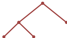
tree
