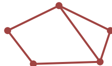
graph
