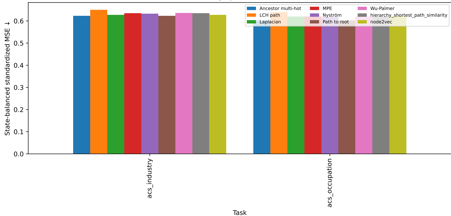
Hierarchy-specific baselines
