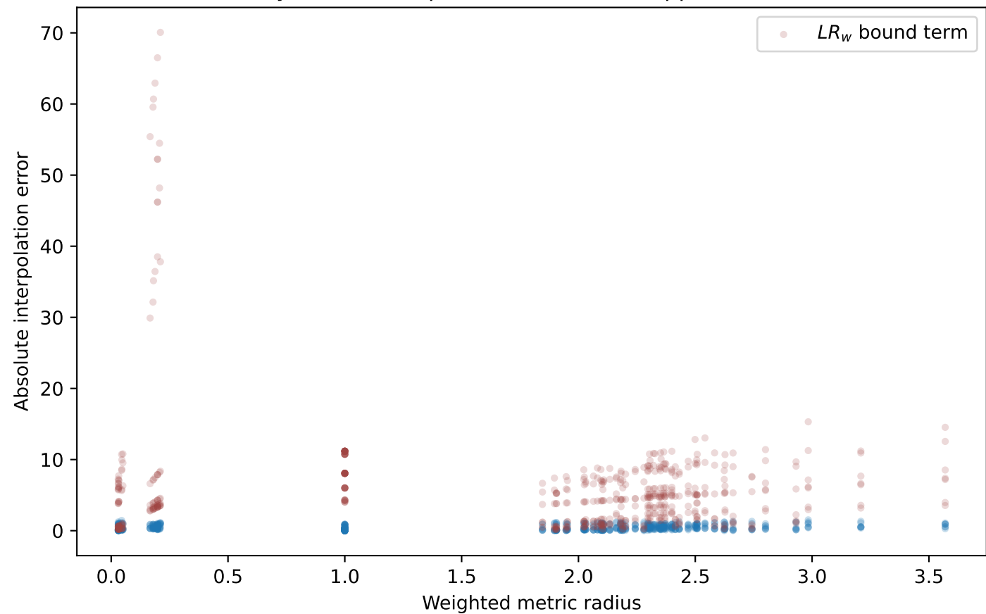
Synthetic interpolation error and support radius
