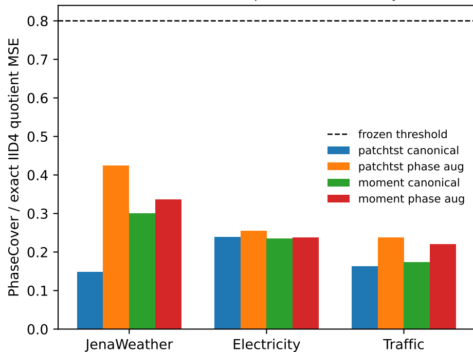
Deterministic quotient efficiency
