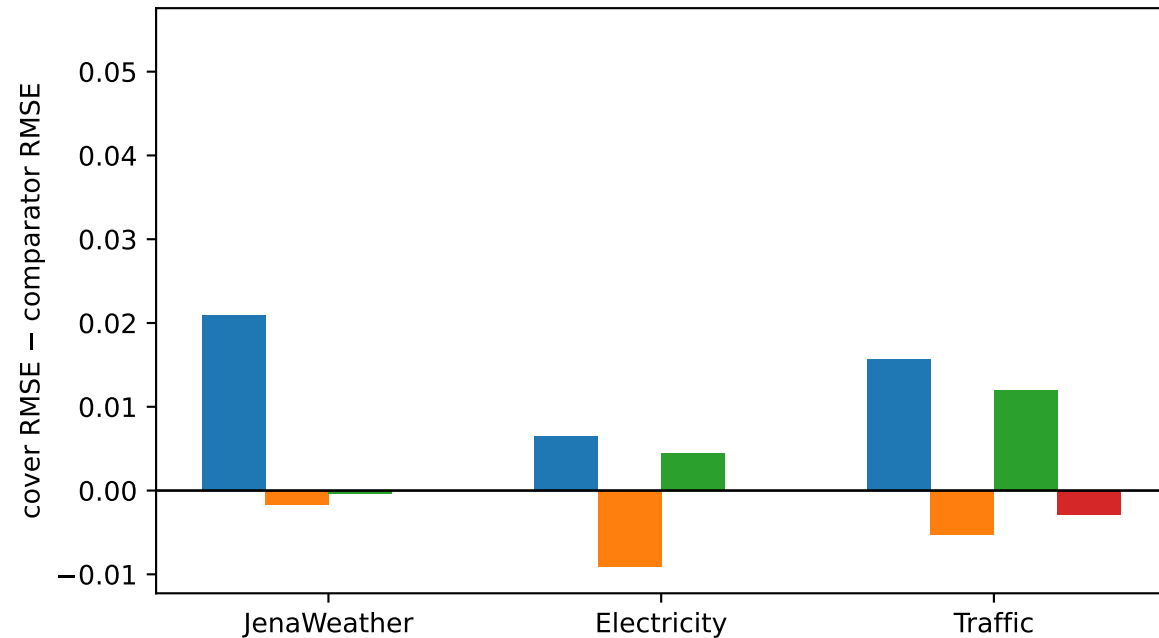
\{0,2,4,6\} vs IID4 containing phase 0
