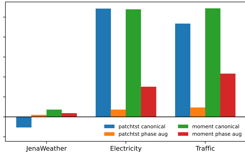
\{1,3,5,7\} vs unconditioned IID4
