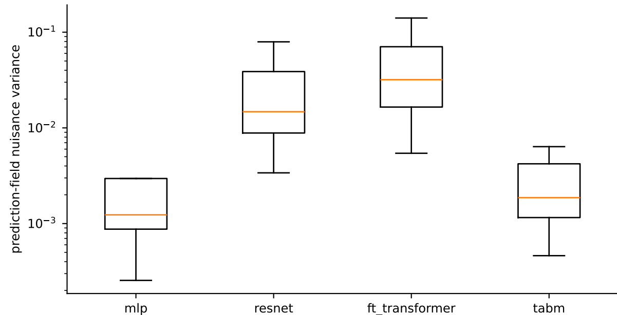
Semantically equivalent representations change fitted predictions
