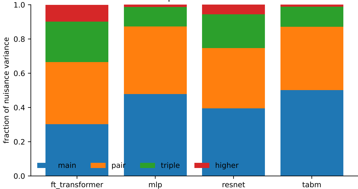
Exact prediction fANOVA
