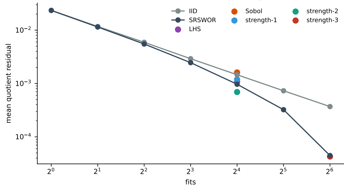
Quotient estimation error versus compute
