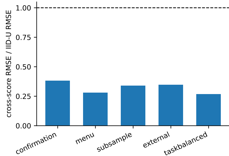
Unbiased quotient-loss estimation
