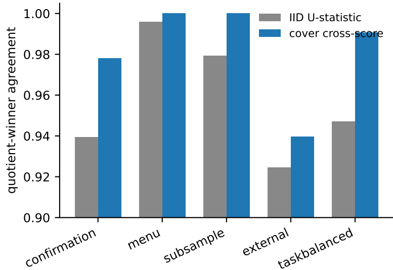
Equal-budget selection (32 fits)
