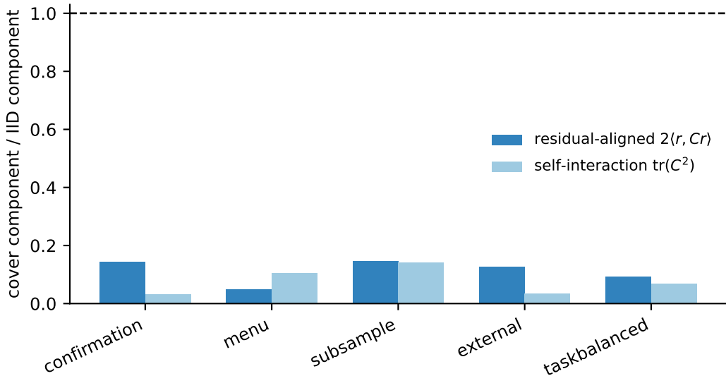
Strength balance reduces both cross-score variance terms
