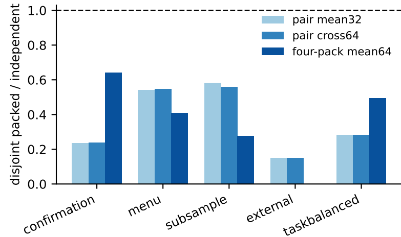
Quotient-score RMSE
