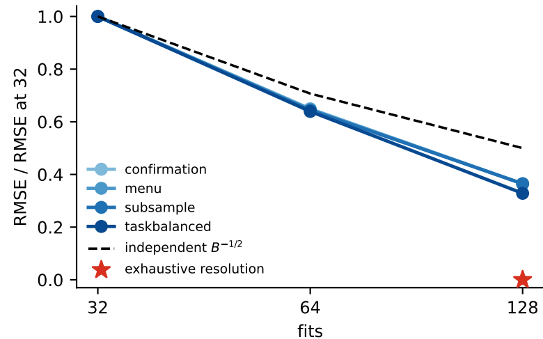
Unbiased packed-score frontier
