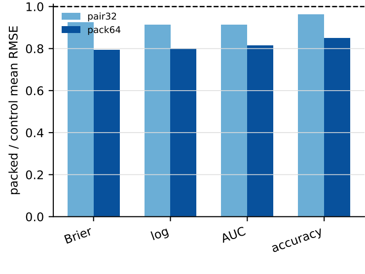
Secondary metric scope
