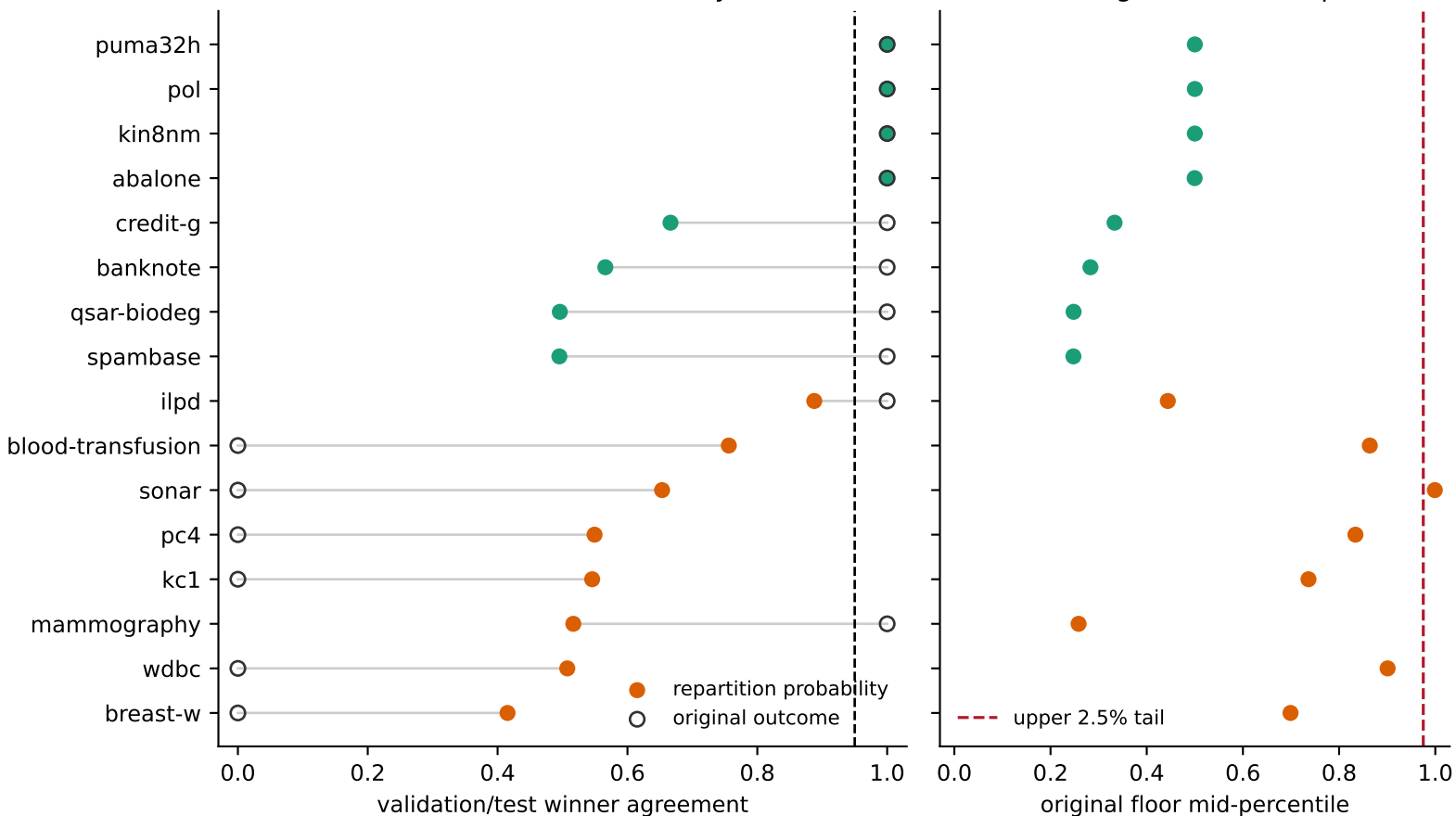
Conditional rank stability
