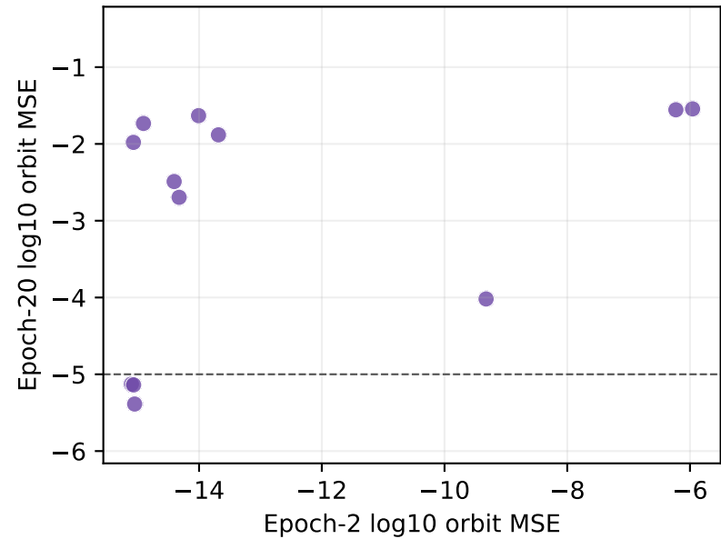
Bank
