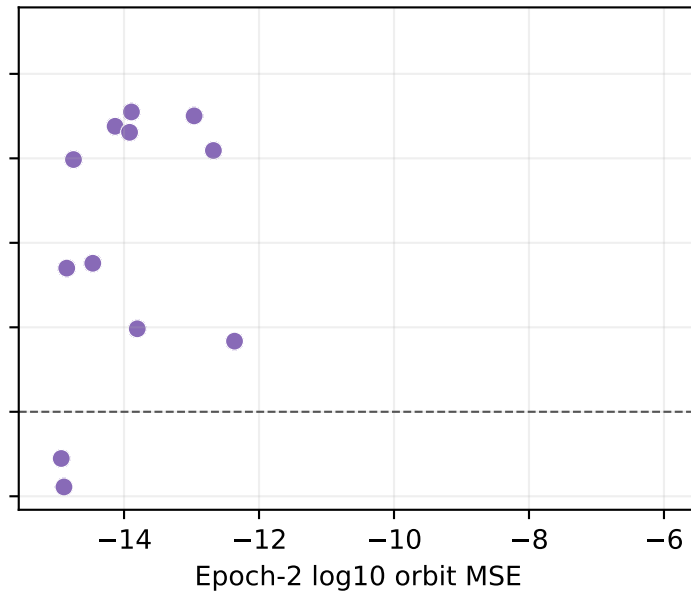
Credit
