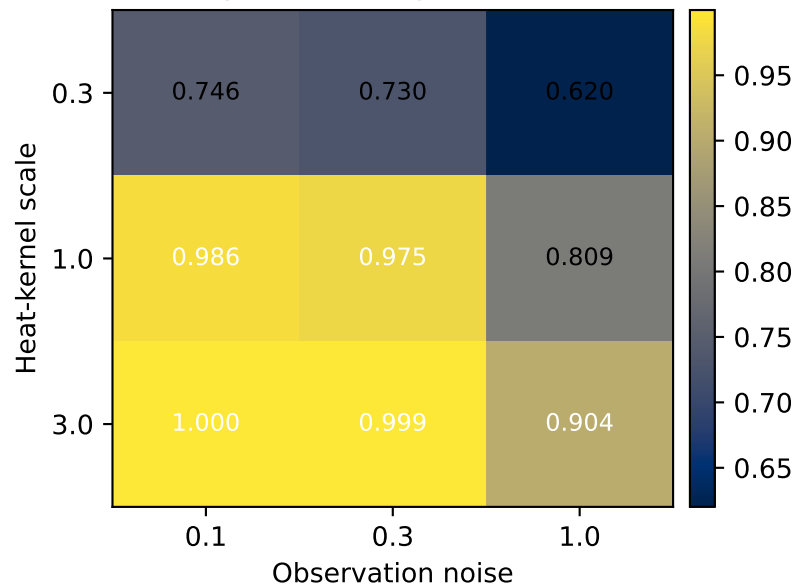
Implicit trust regime AUROC
