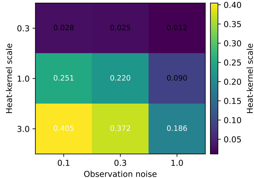
Gain over geometry-free transformer
