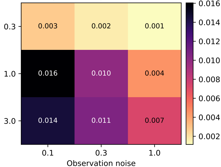
Regret to analytic Bayes rule
