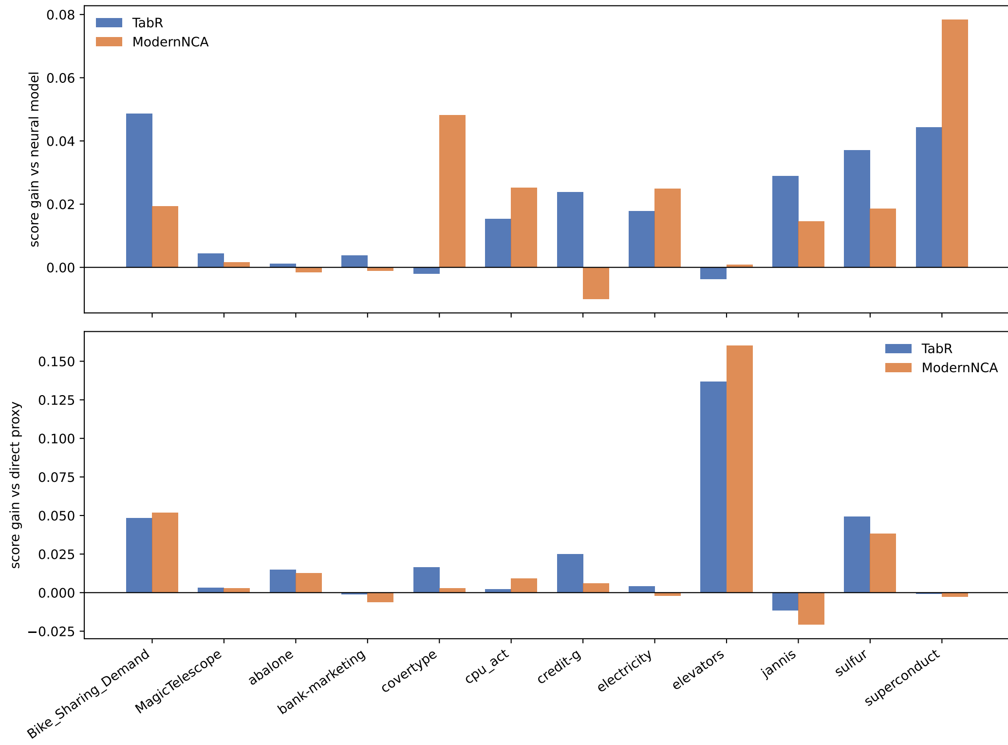
Post-hoc full aggregate-risk weighting
