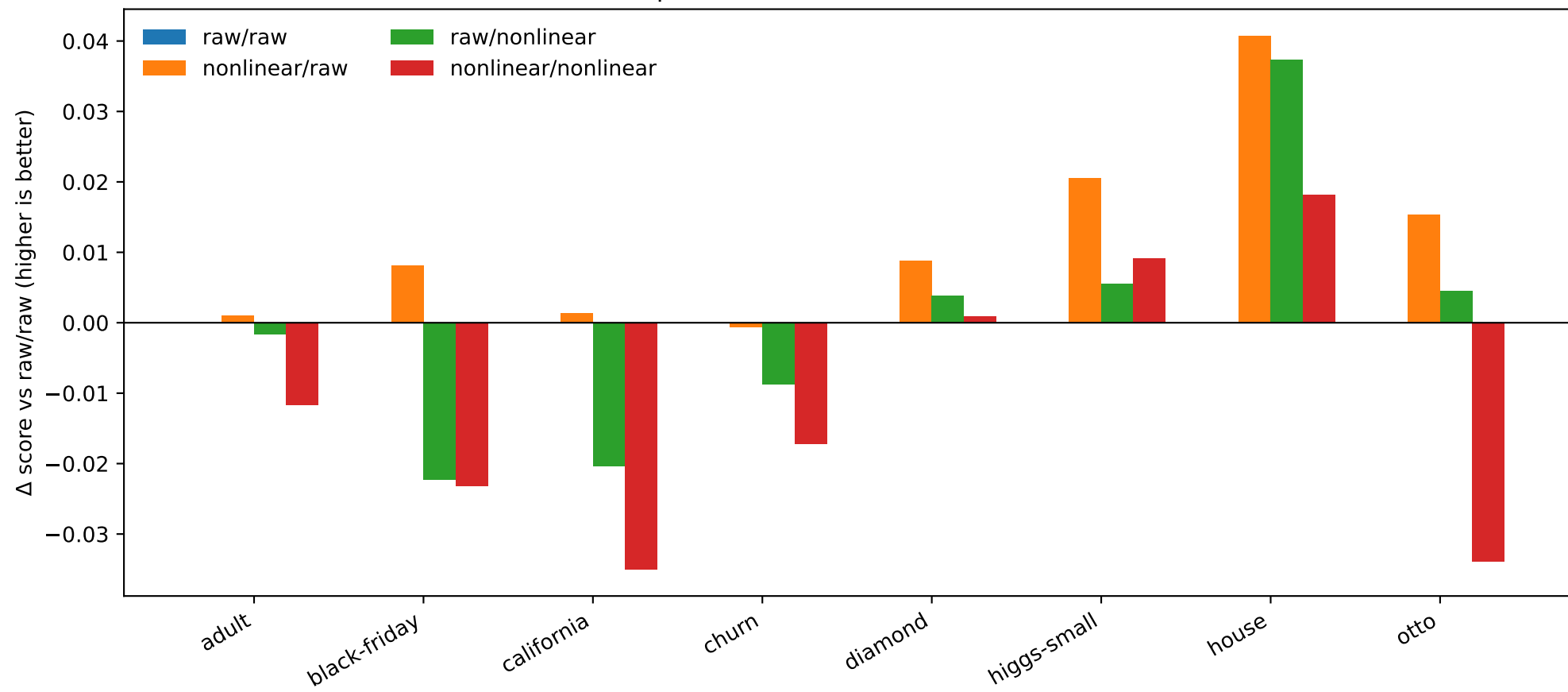
TabR prediction/retrieval branch ablation
