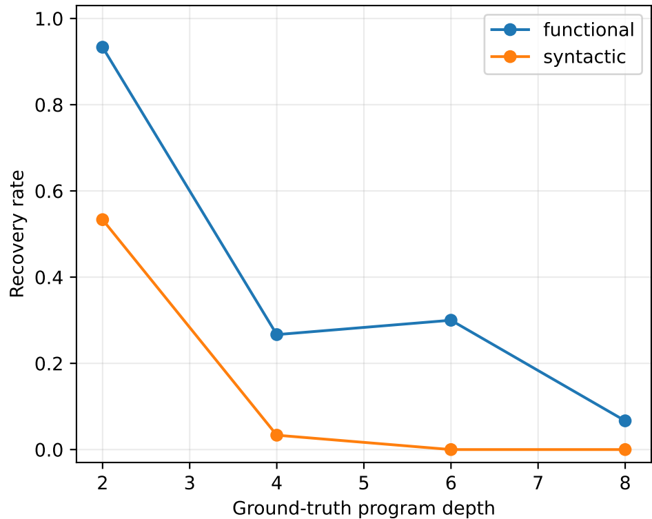
Depth scaling separates execution from discovery
